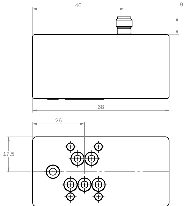
Mating Pattern
