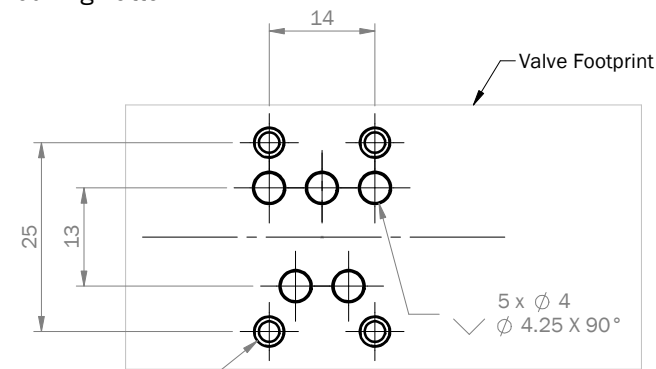
Mating Pattern
